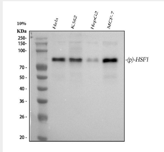
Figure 1. Western blot analysis of HSF1 using anti-HSF1 antibody (P00250).
